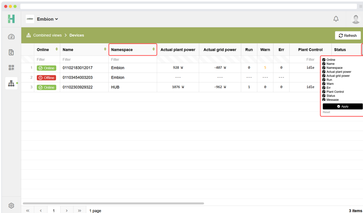
Figure 125: Devices combined view filter options
